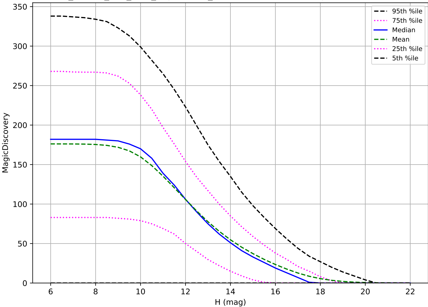
ddf_loaded_fl15_v3.4_10yrs: OCC_r5 6 detections in 60 nights detection loss
