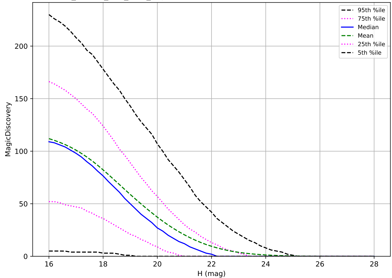
ddf_loaded_fl15_v3.4_10yrs: NEO 6 detections in 60 nights detection loss
