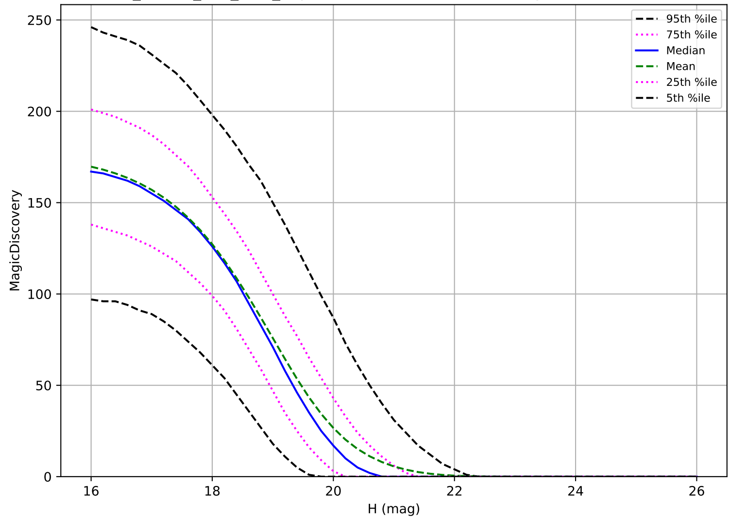
ddf_loaded_fl15_v3.4_10yrs: MBA 6 detections in 60 nights detection loss
