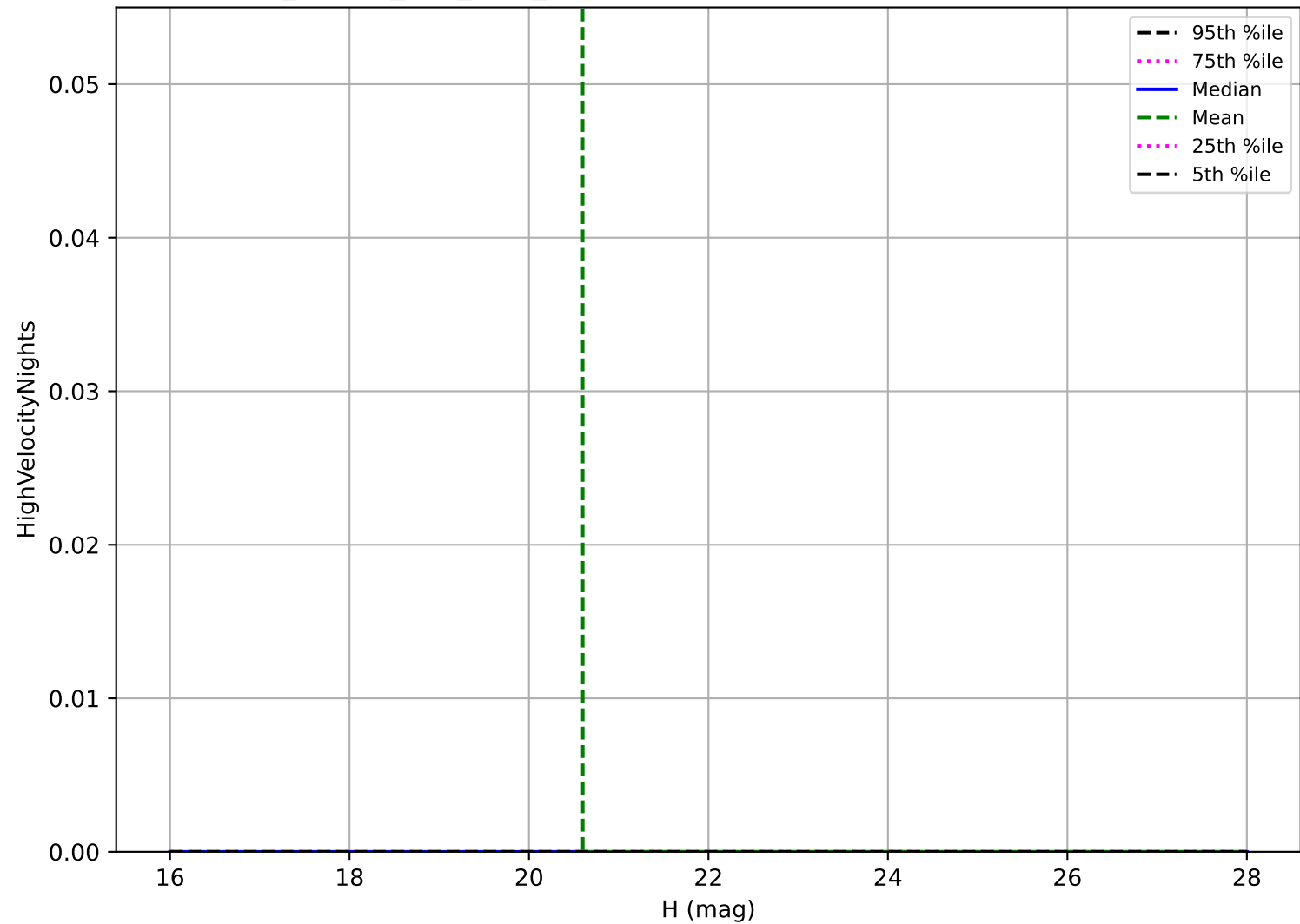
ddf_loaded_fl15_v3.4_10yrs: Vatira High velocity pair detection loss
