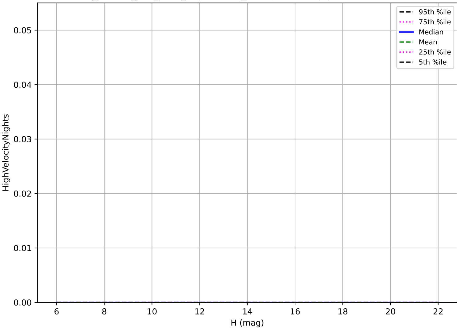
ddf_loaded_fl15_v3.4_10yrs: OCC_r5 High velocity pair detection loss
