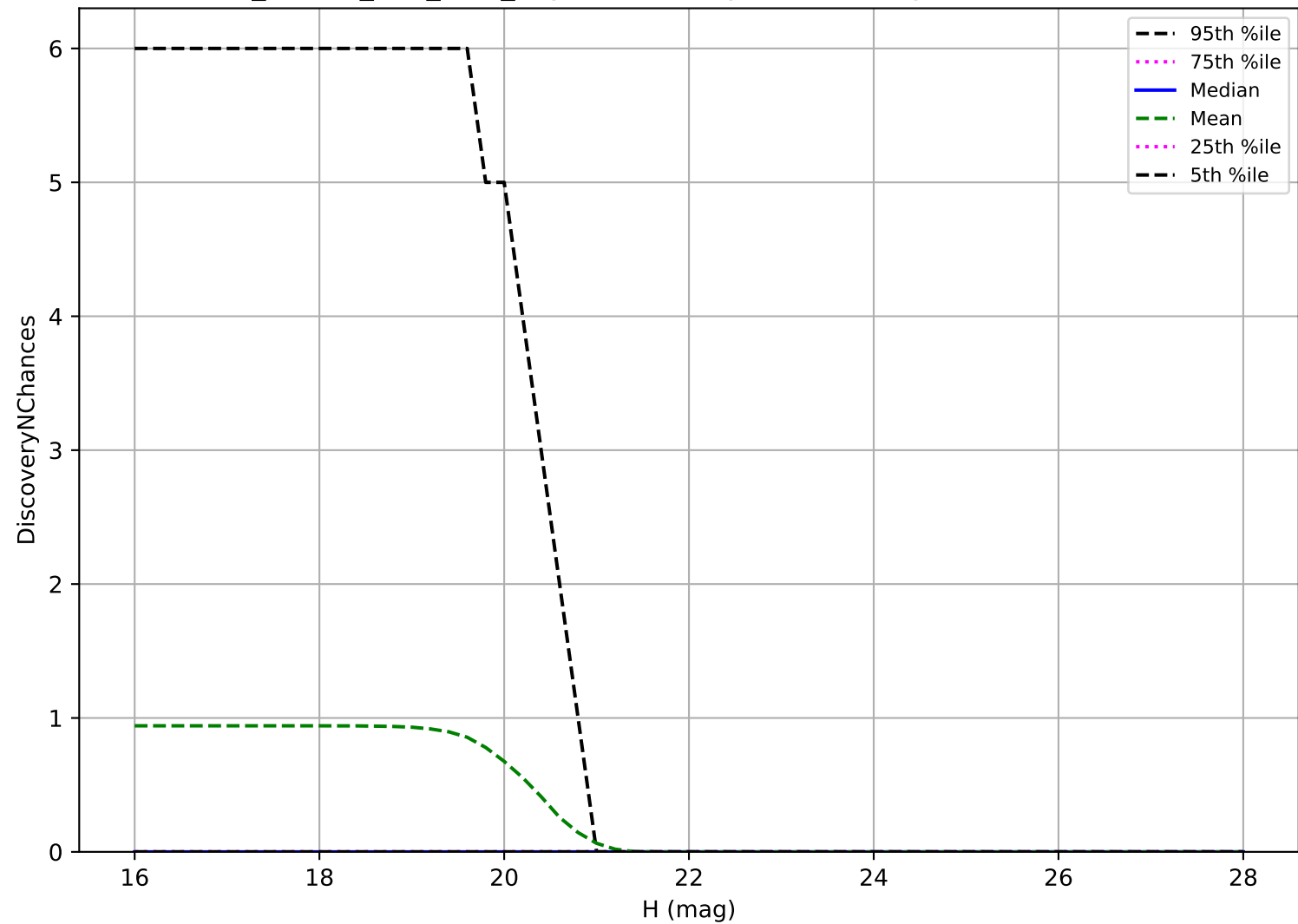
ddf_loaded_fl15_v3.4_10yrs: Vatira 3 pairs in 15 nights detection loss
