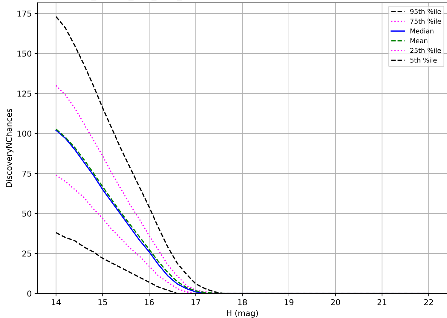
ddf_loaded_fl15_v3.4_10yrs: Trojan 3 pairs in 15 nights detection loss
