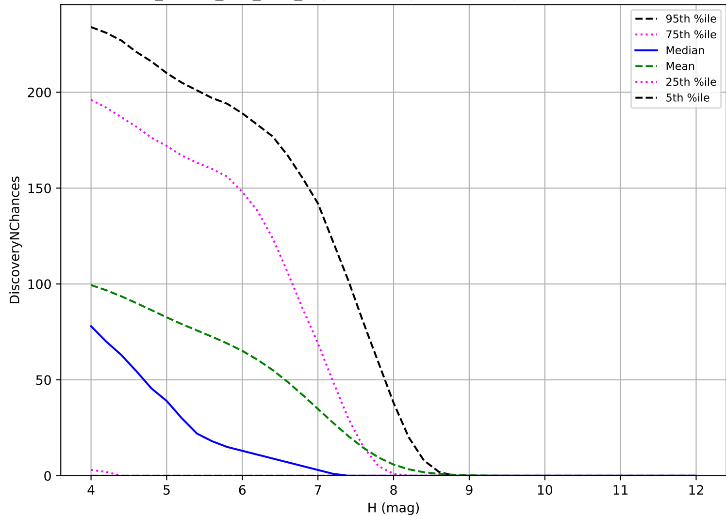
ddf_loaded_fl15_v3.4_10yrs: TNO 3 pairs in 15 nights detection loss
