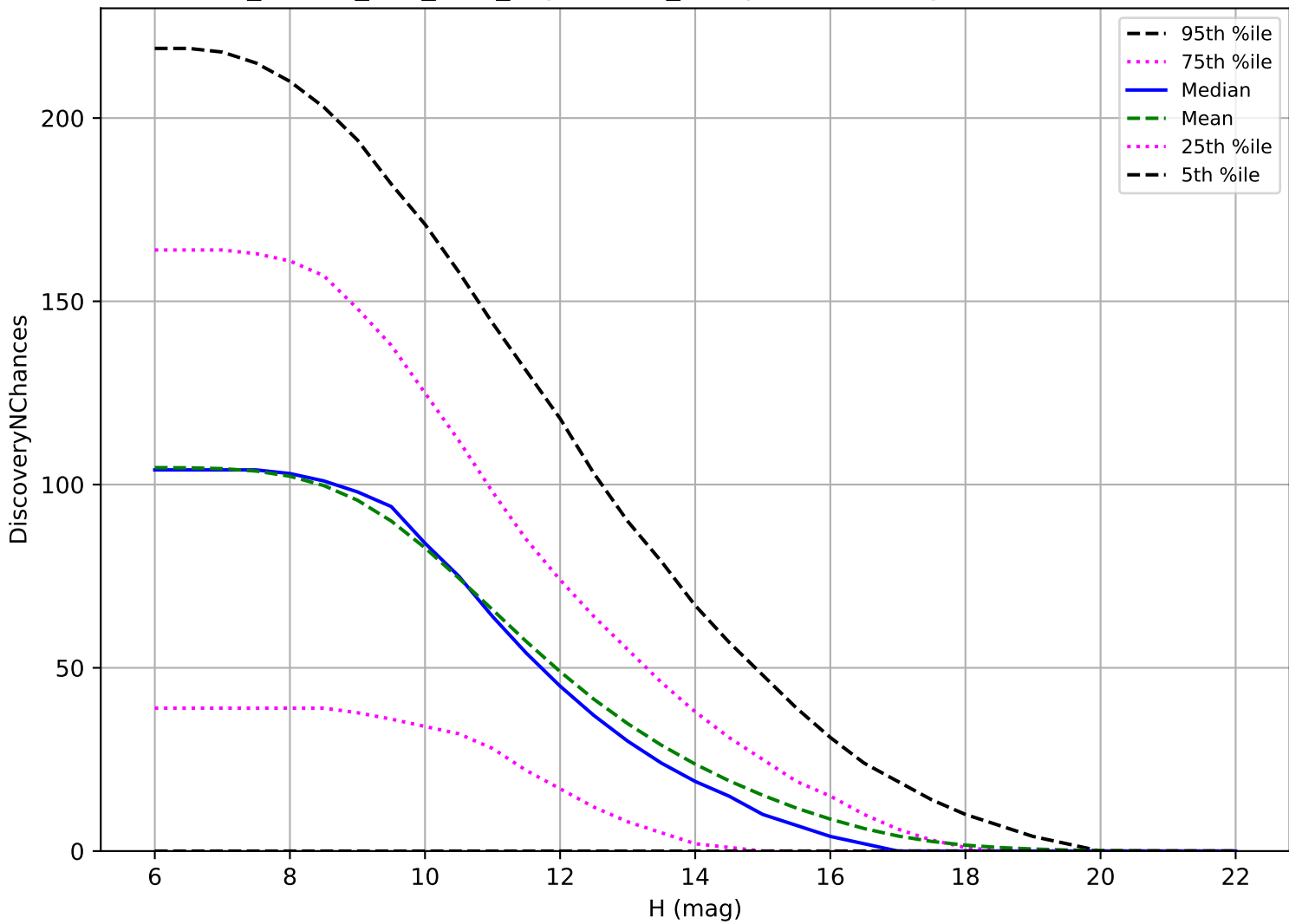
ddf_loaded_fl15_v3.4_10yrs: OCC_r5 3 pairs in 15 nights detection loss
