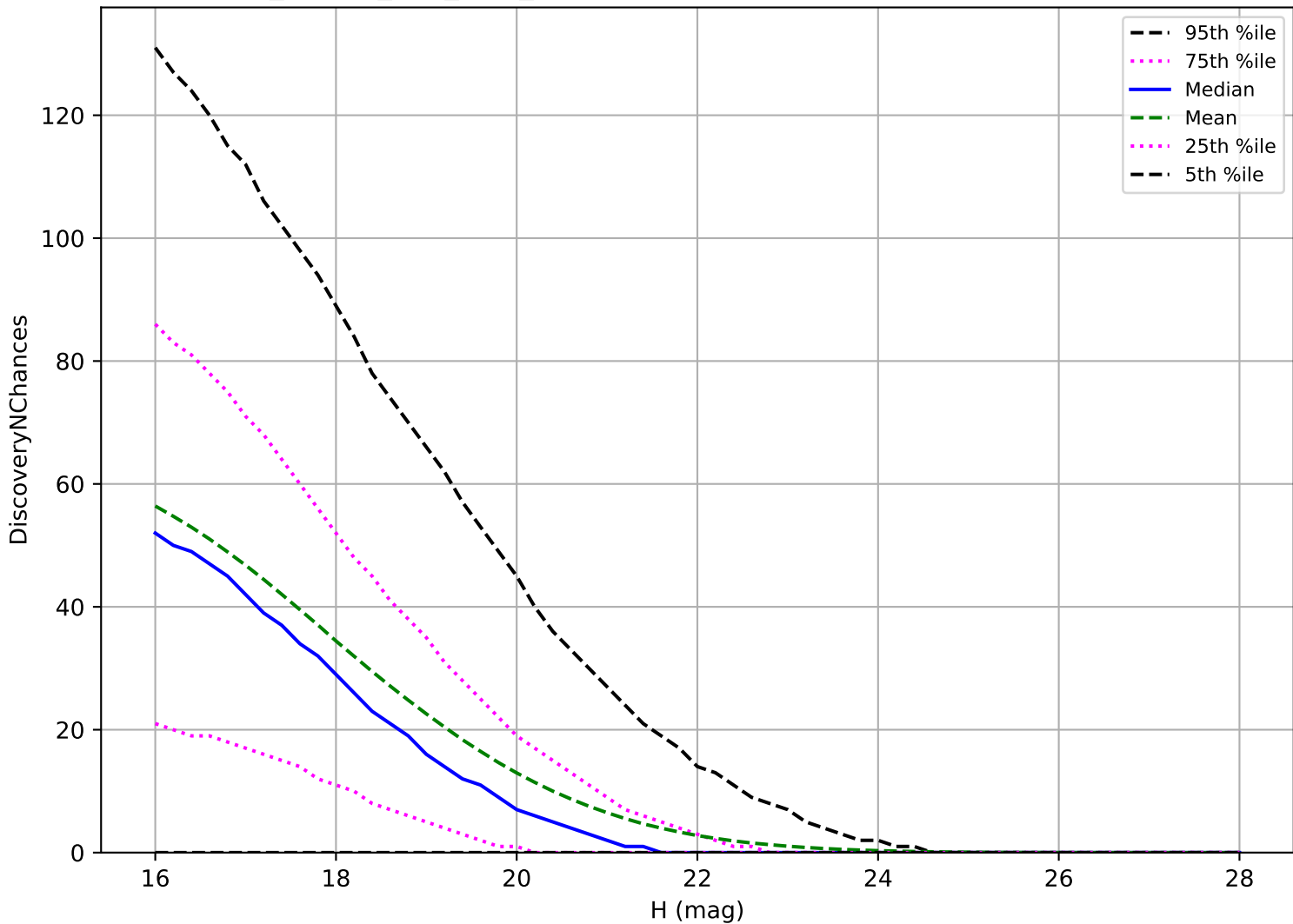
ddf_loaded_fl15_v3.4_10yrs: NEO 3 pairs in 15 nights detection loss
