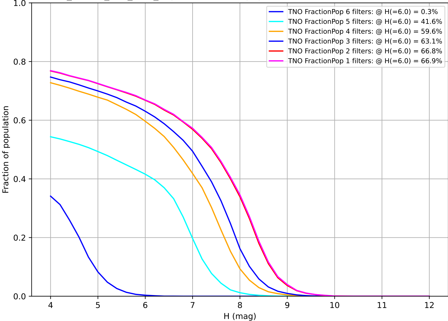
ddf_loaded_fl15_v3.4_10yrs: Fraction of population with colors in X filters TNO
