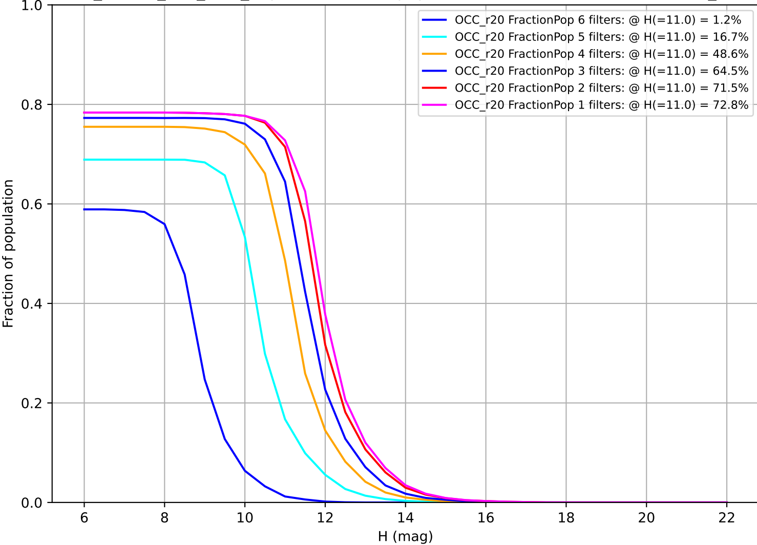
ddf_loaded_fl15_v3.4_10yrs: Fraction of population with colors in X filters OCC_r20
