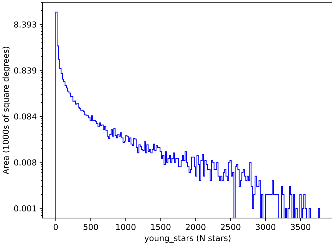
ddf_loaded_fl15_v3.4_10yrs : young_stars
