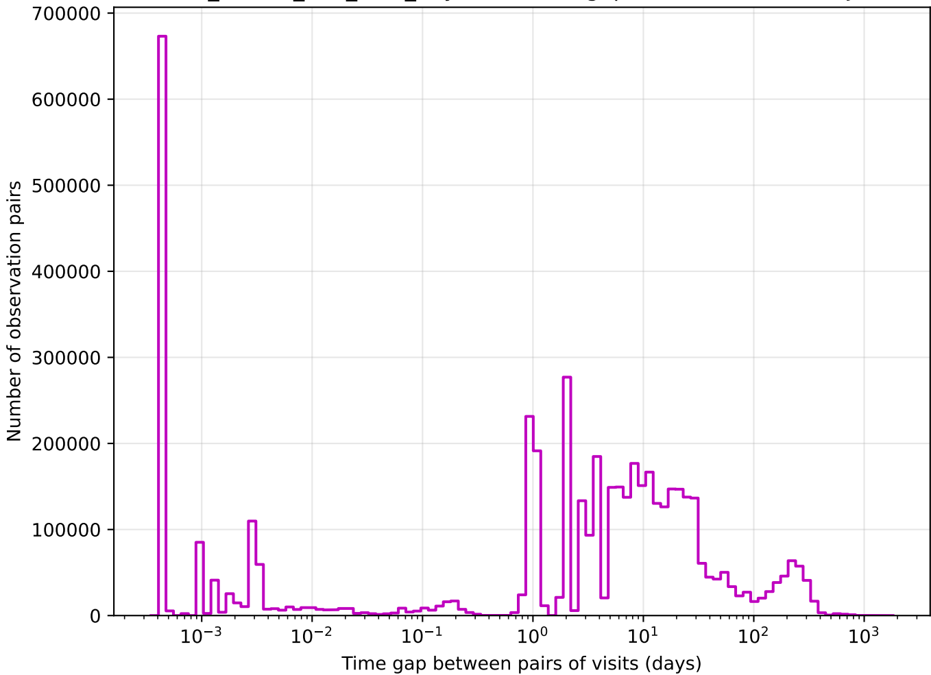
ddf_loaded_fl15_v3.4_10yrs z band: Tgaps observationStartMJD
