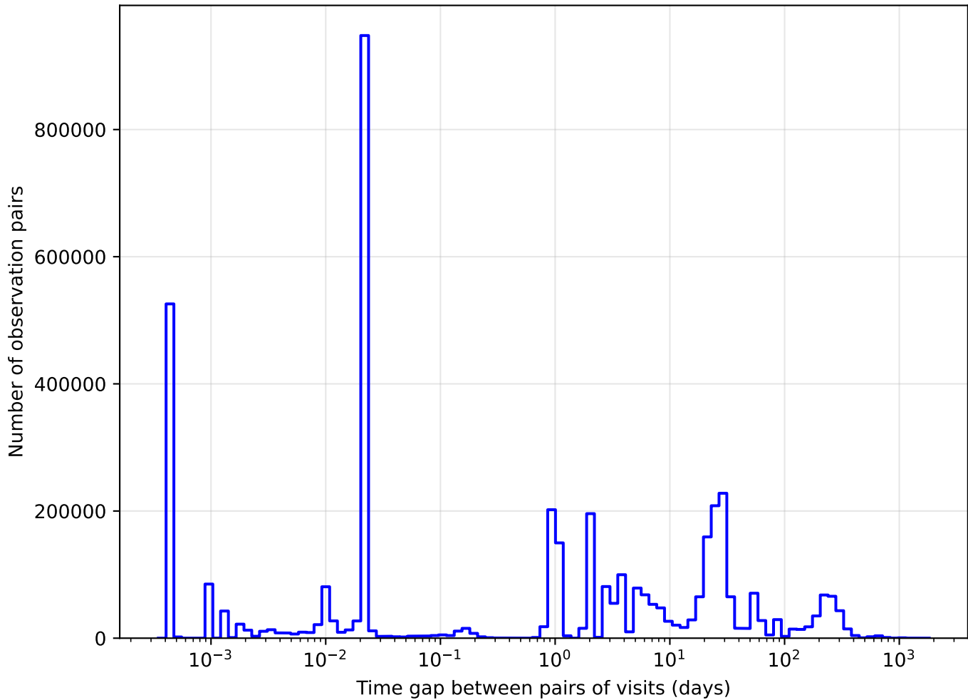
ddf_loaded_fl15_v3.4_10yrs y band: Tgaps observationStartMJD
