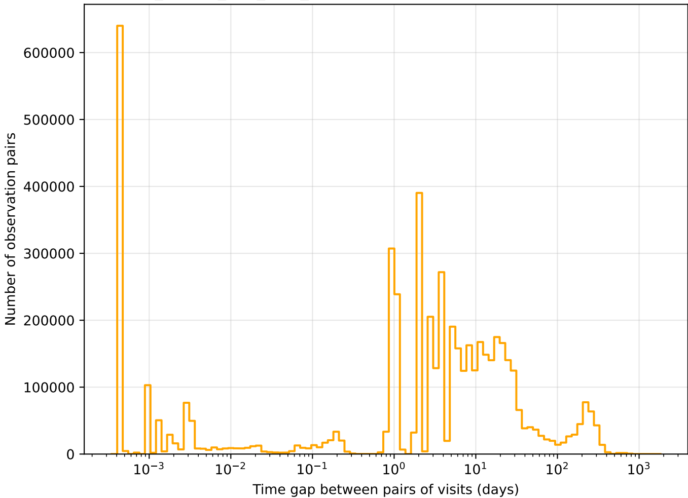
ddf_loaded_fl15_v3.4_10yrs r band: Tgaps observationStartMJD
