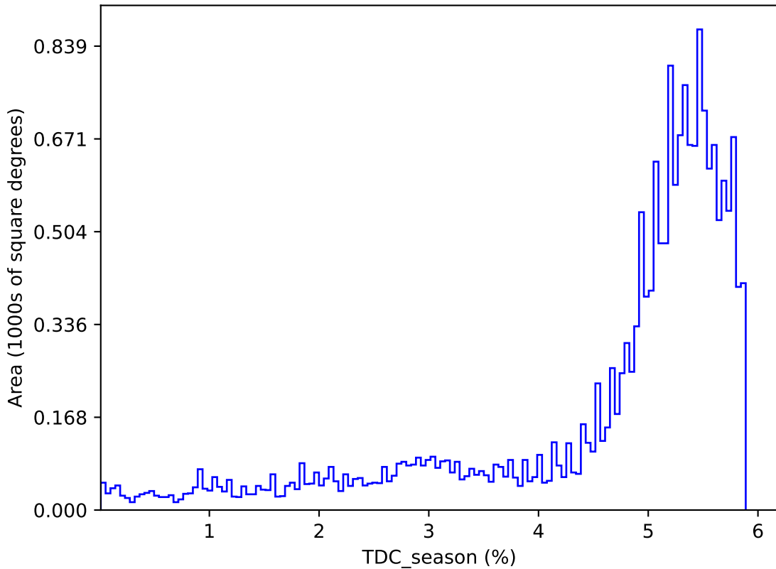
ddf_loaded_fl15_v3.4_10yrs : TDC_season
