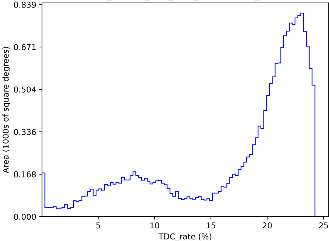
ddf_loaded_fl15_v3.4_10yrs : TDC_rate
