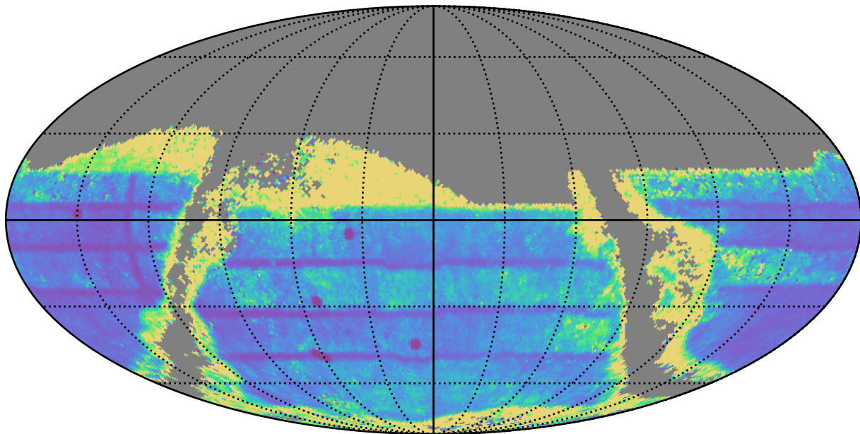
ddf_loaded_fl15_v3.4_10yrs : TDC_cadence
