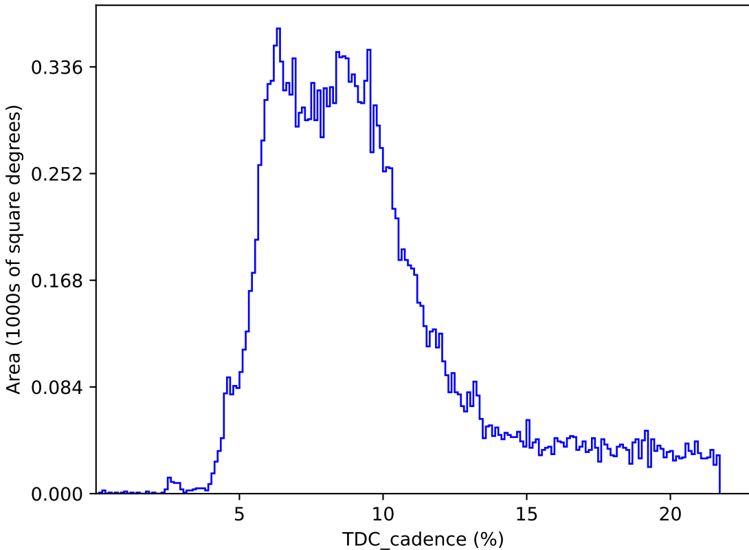
ddf_loaded_fl15_v3.4_10yrs : TDC_cadence
