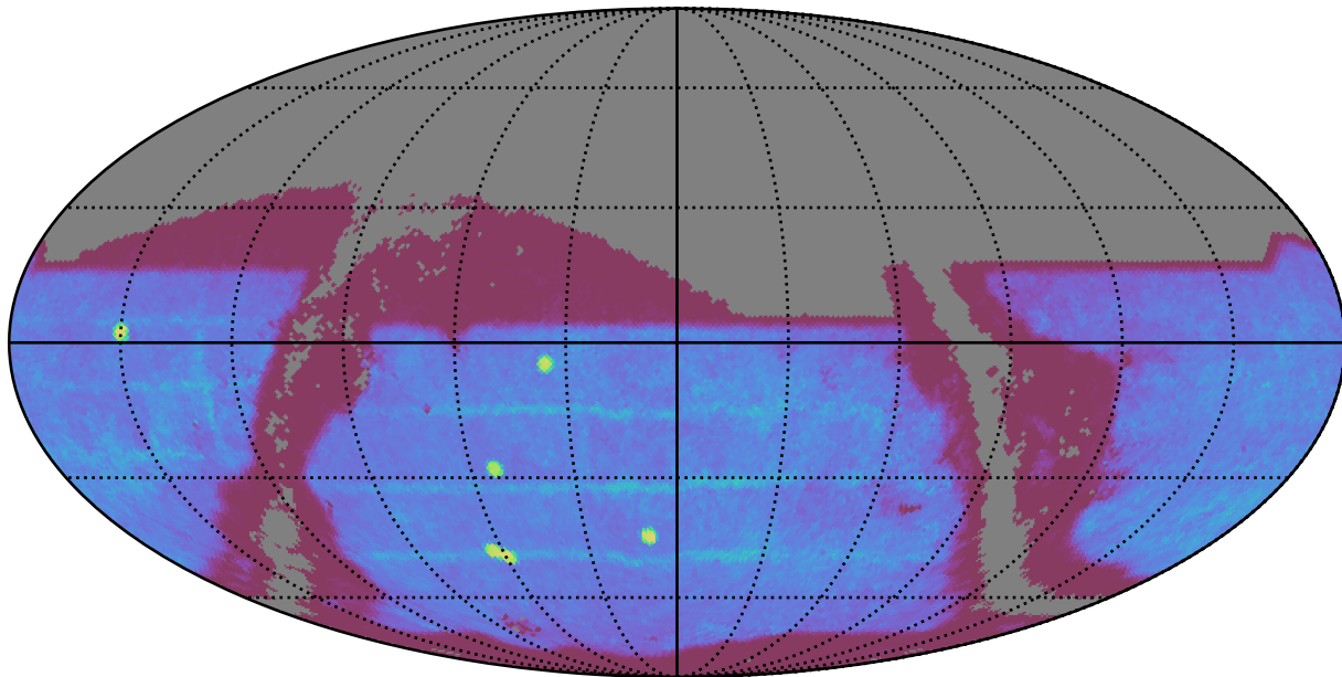
ddf_loaded_fl15_v3.4_10yrs : SNSLMetric
