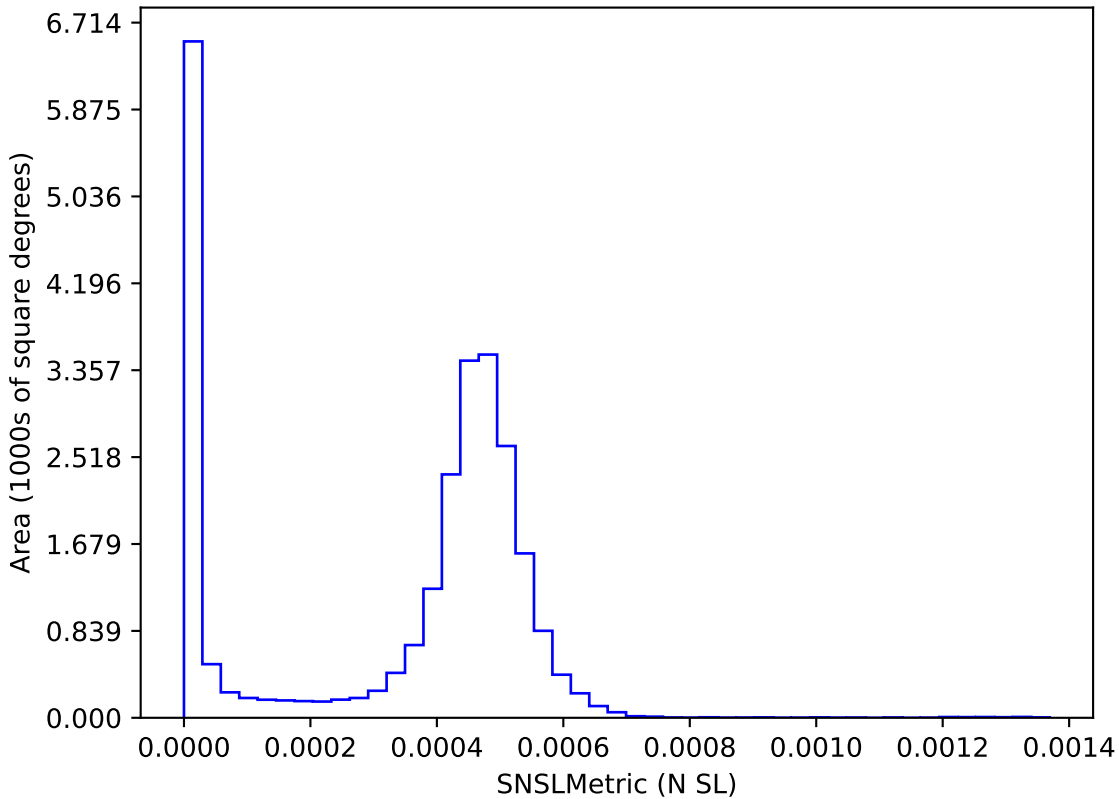
ddf_loaded_fl15_v3.4_10yrs : SNSLMetric
