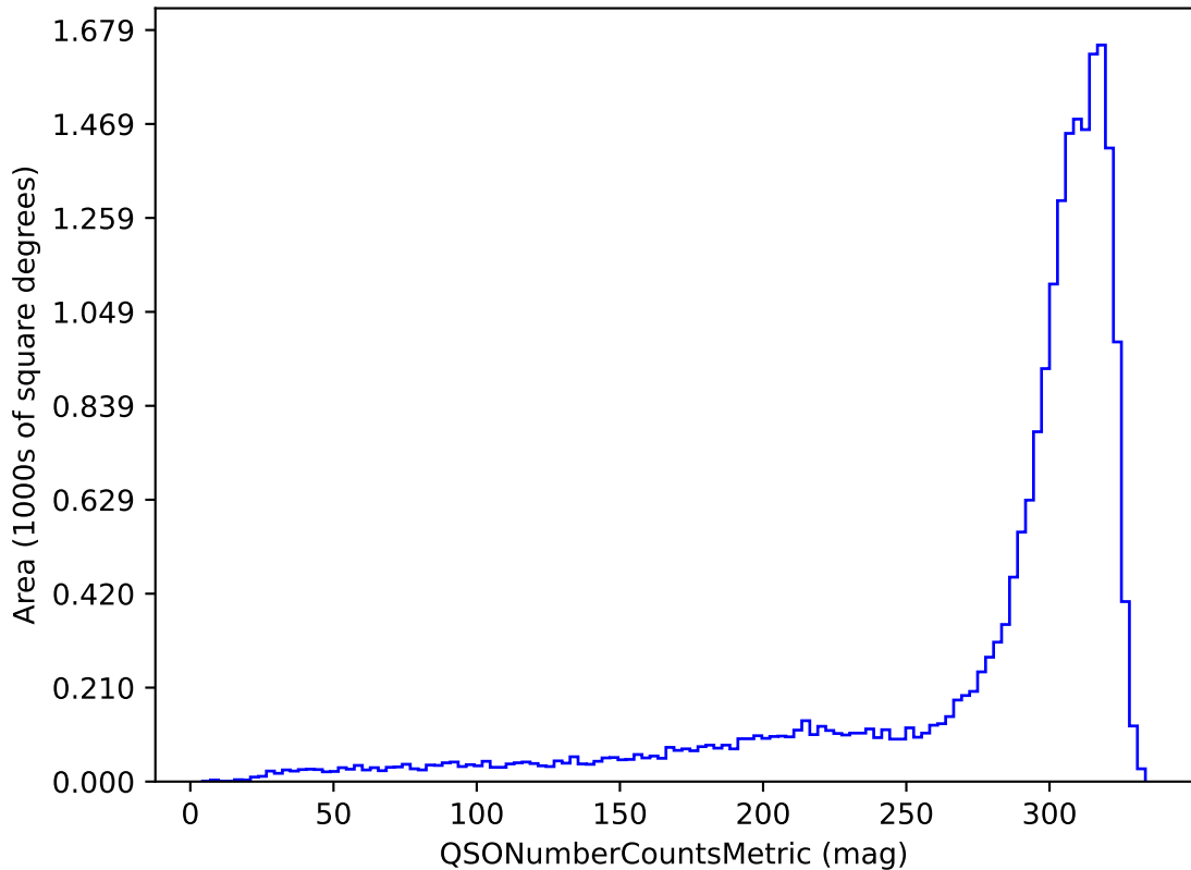
ddf_loaded_fl15_v3.4_10yrs u band and non-DD: QSONumberCountsMetric
