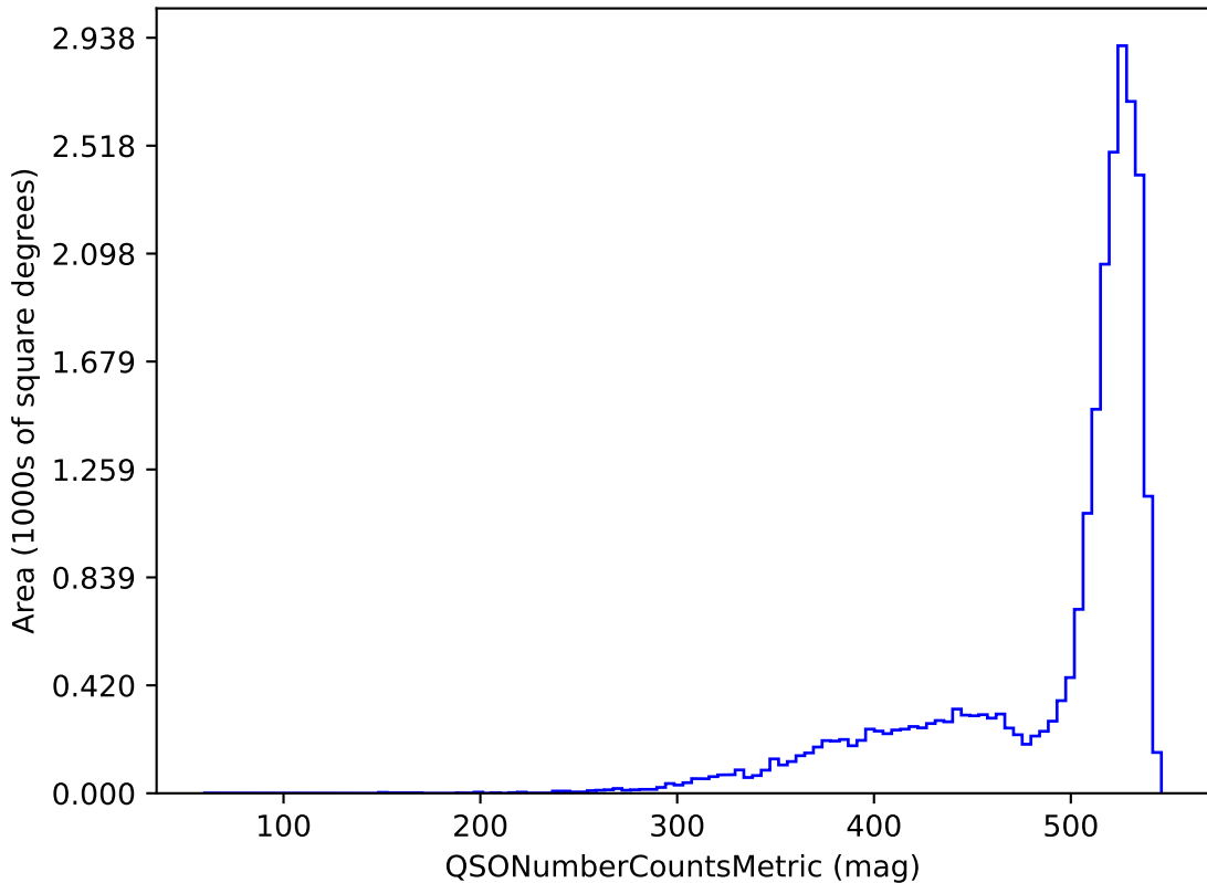
ddf_loaded_fl15_v3.4_10yrs r band and non-DD: QSONumberCountsMetric
