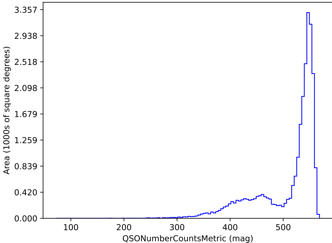
ddf_loaded_fl15_v3.4_10yrs i band and non-DD: QSONumberCountsMetric
