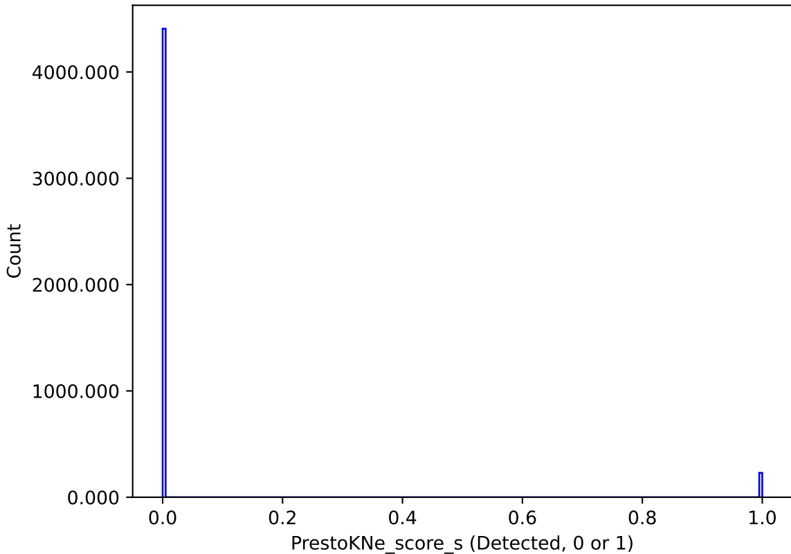
ddf_loaded_fl15_v3.4_10yrs : PrestoKNe_score_s
