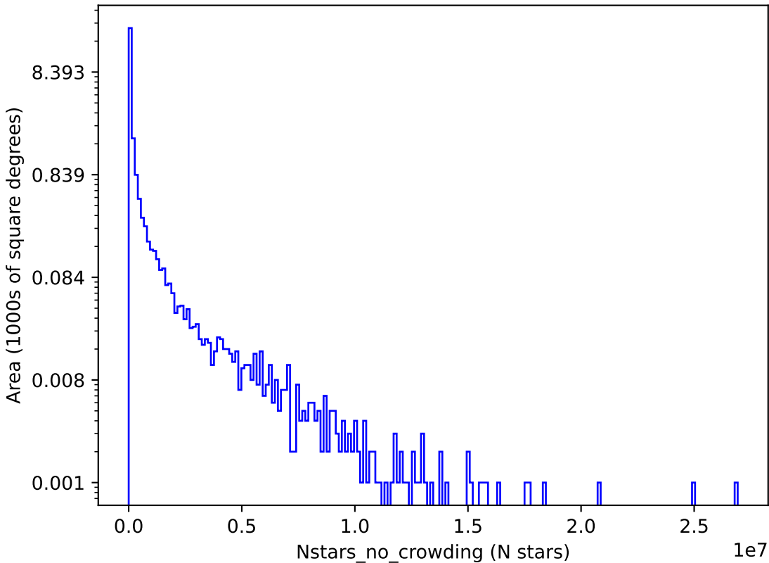
ddf_loaded_fl15_v3.4_10yrs z: Nstars_no_crowding
