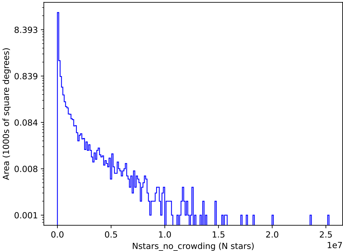
ddf_loaded_fl15_v3.4_10yrs y: Nstars_no_crowding
