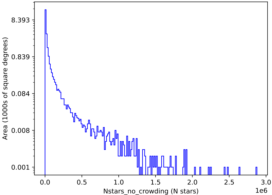
ddf_loaded_fl15_v3.4_10yrs u: Nstars_no_crowding
