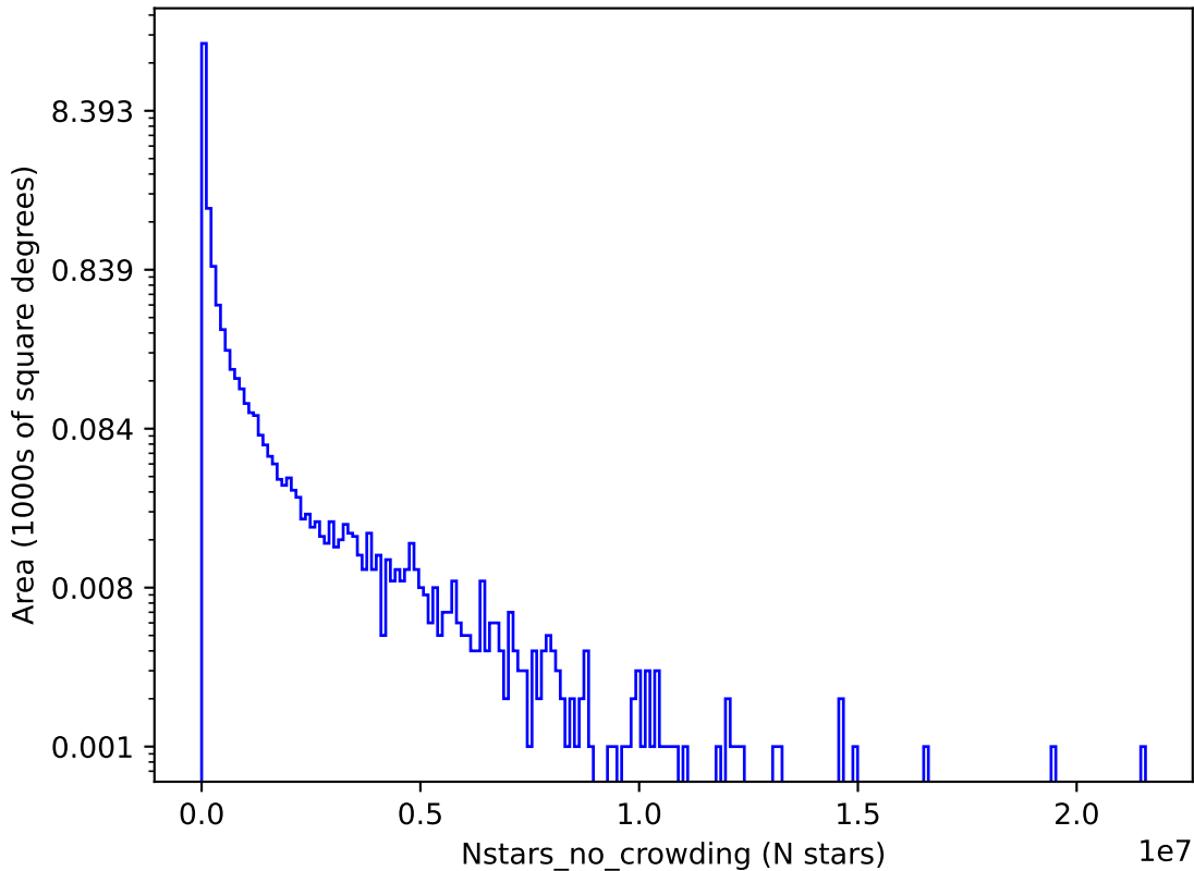
ddf_loaded_fl15_v3.4_10yrs r: Nstars_no_crowding
