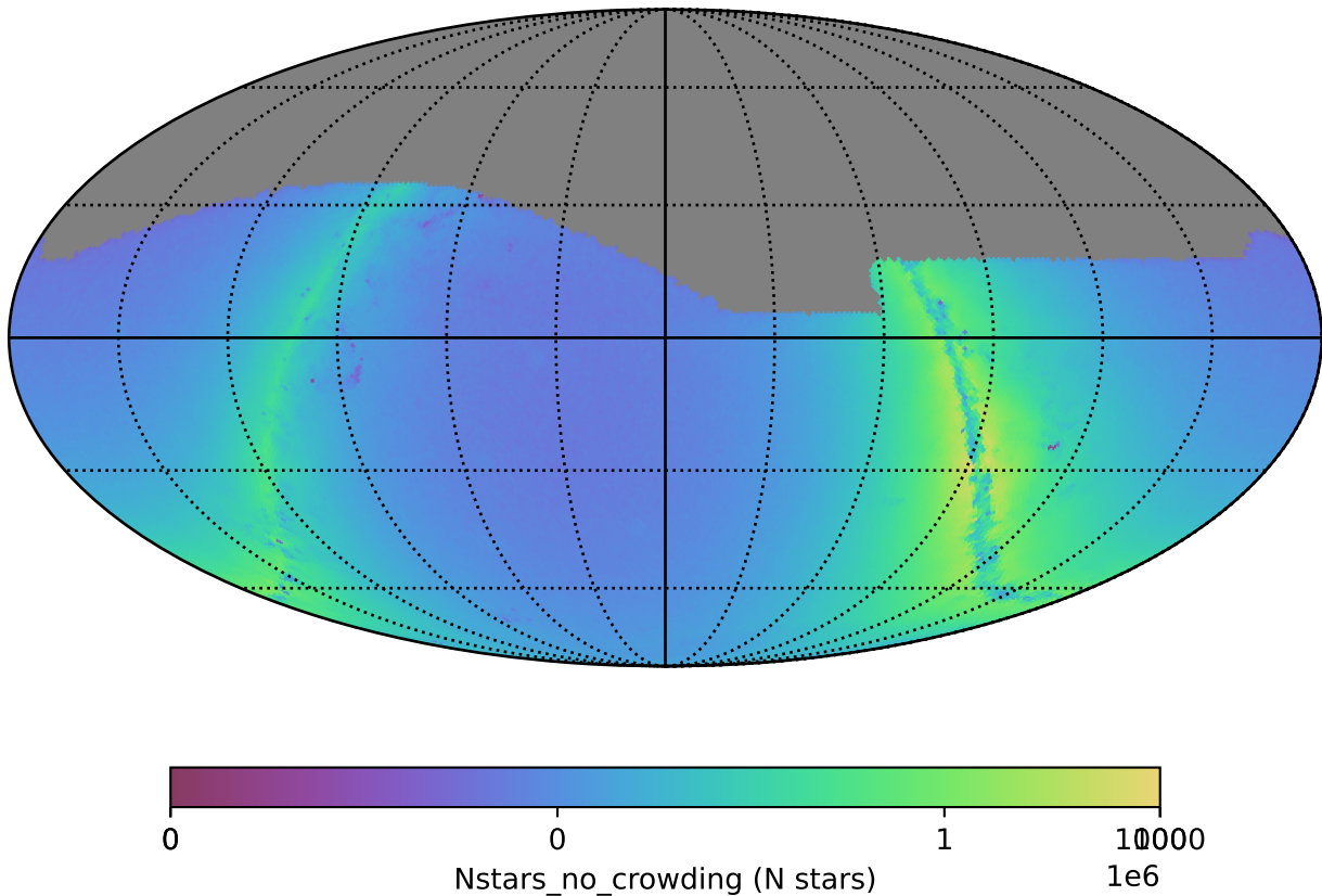
ddf_loaded_fl15_v3.4_10yrs g: Nstars_no_crowding
