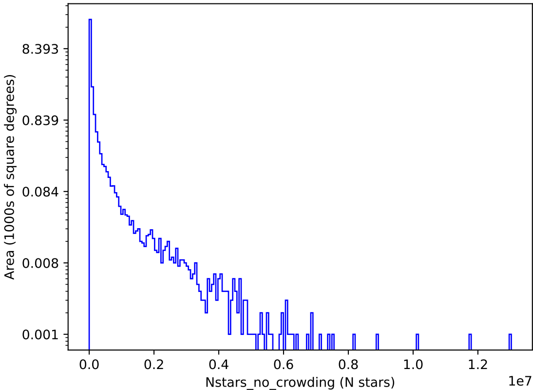
ddf_loaded_fl15_v3.4_10yrs g: Nstars_no_crowding
