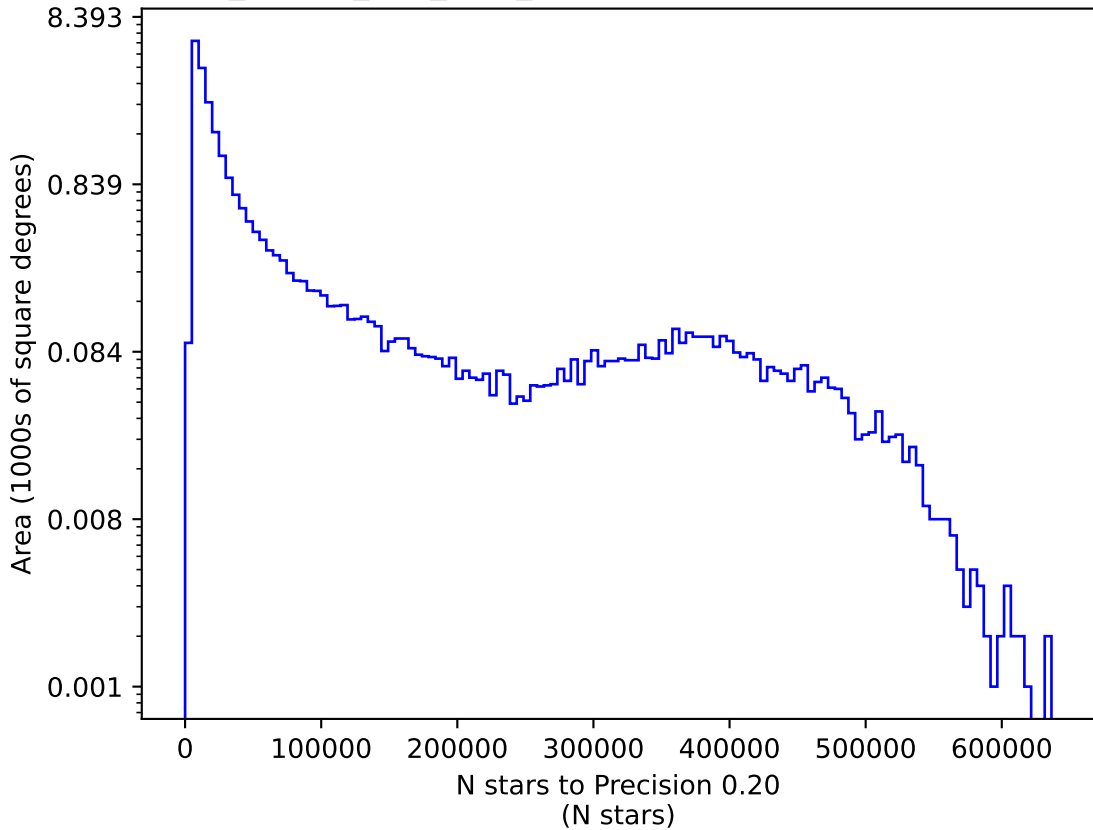
ddf_loaded_fl15_v3.4_10yrs z: N stars to Precision 0.20
