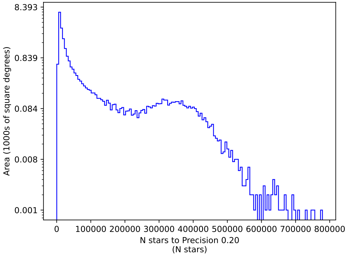
ddf_loaded_fl15_v3.4_10yrs y: N stars to Precision 0.20
