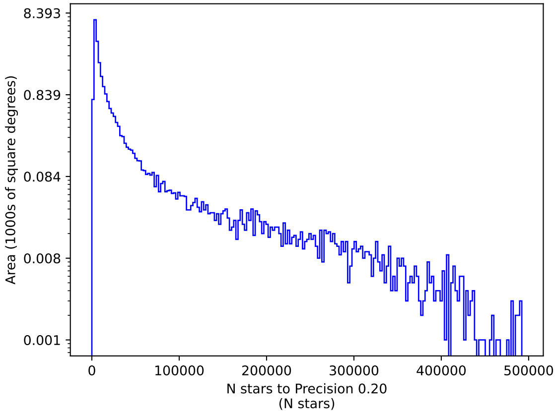
ddf_loaded_fl15_v3.4_10yrs u: N stars to Precision 0.20
