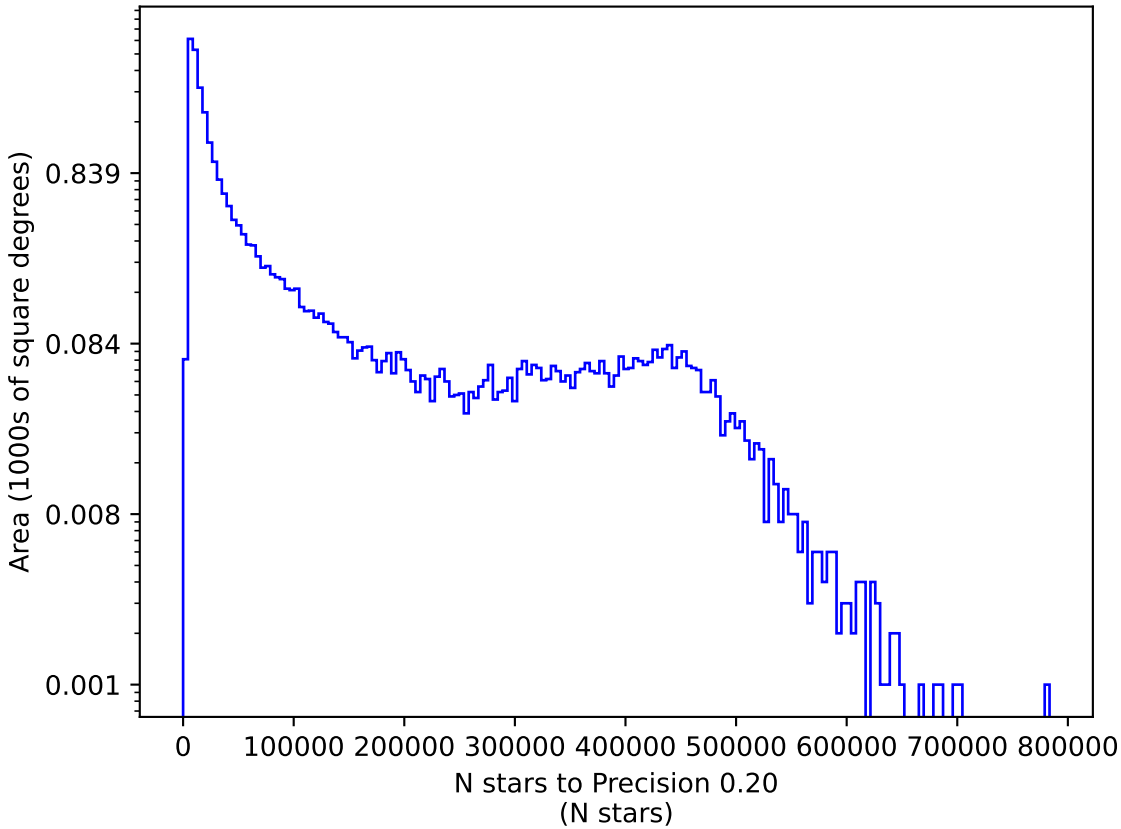
ddf_loaded_fl15_v3.4_10yrs r: N stars to Precision 0.20
