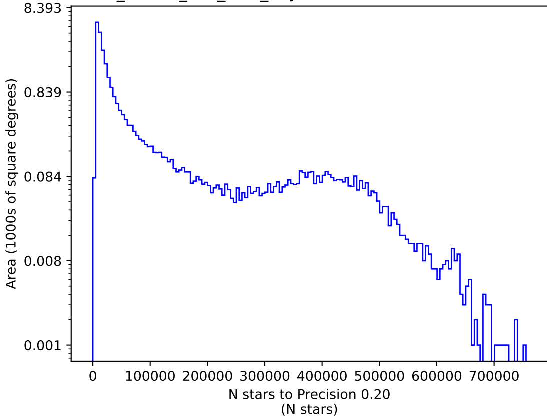
ddf_loaded_fl15_v3.4_10yrs i: N stars to Precision 0.20
