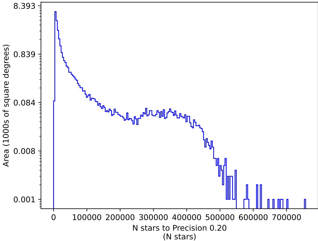
ddf_loaded_fl15_v3.4_10yrs g: N stars to Precision 0.20
