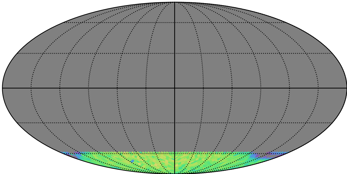
ddf_loaded_fl15_v3.4_10yrs gi SCP: LVDwarfs
