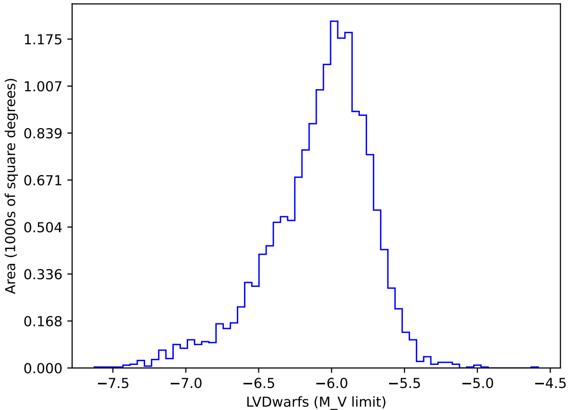
ddf_loaded_fl15_v3.4_10yrs gi: LVDwarfs
