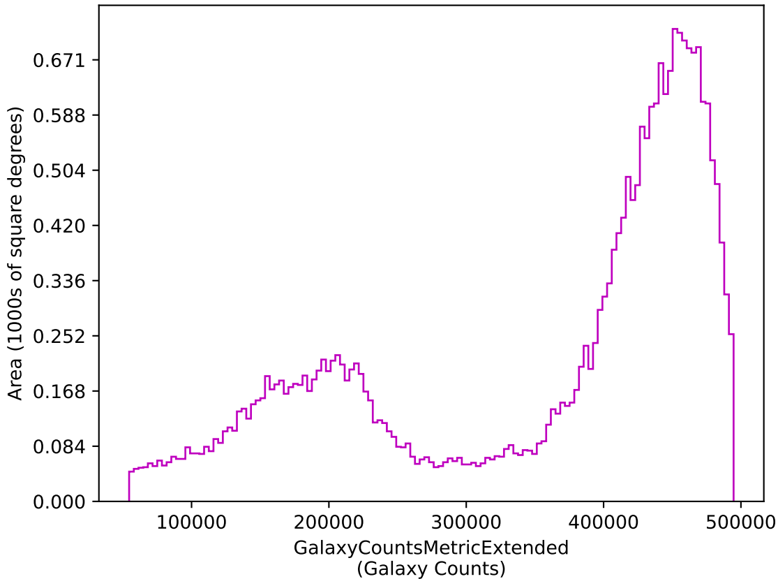
ddf_loaded_fl15_v3.4_10yrs z: GalaxyCountsMetricExtended
