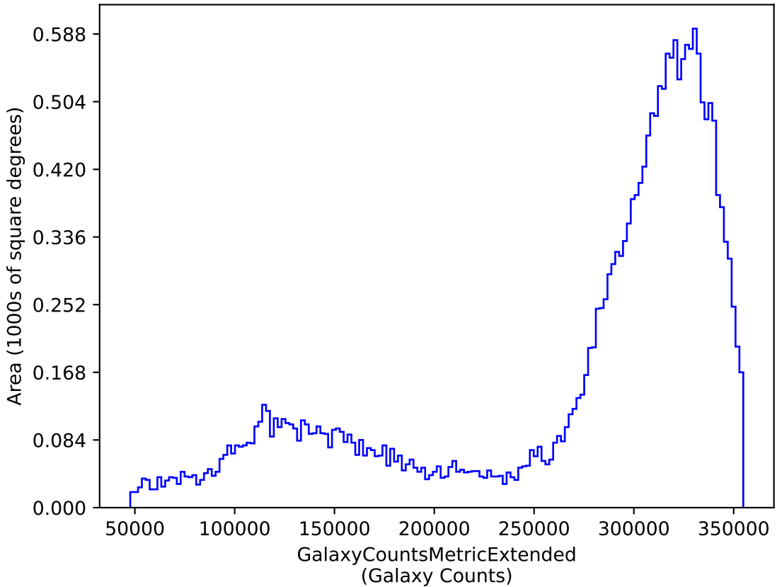
ddf_loaded_fl15_v3.4_10yrs y: GalaxyCountsMetricExtended
