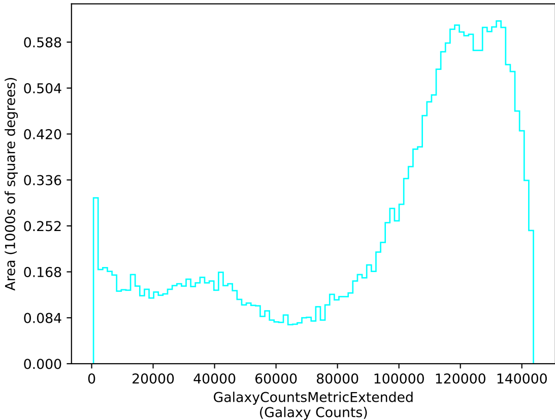
ddf_loaded_fl15_v3.4_10yrs u: GalaxyCountsMetricExtended
