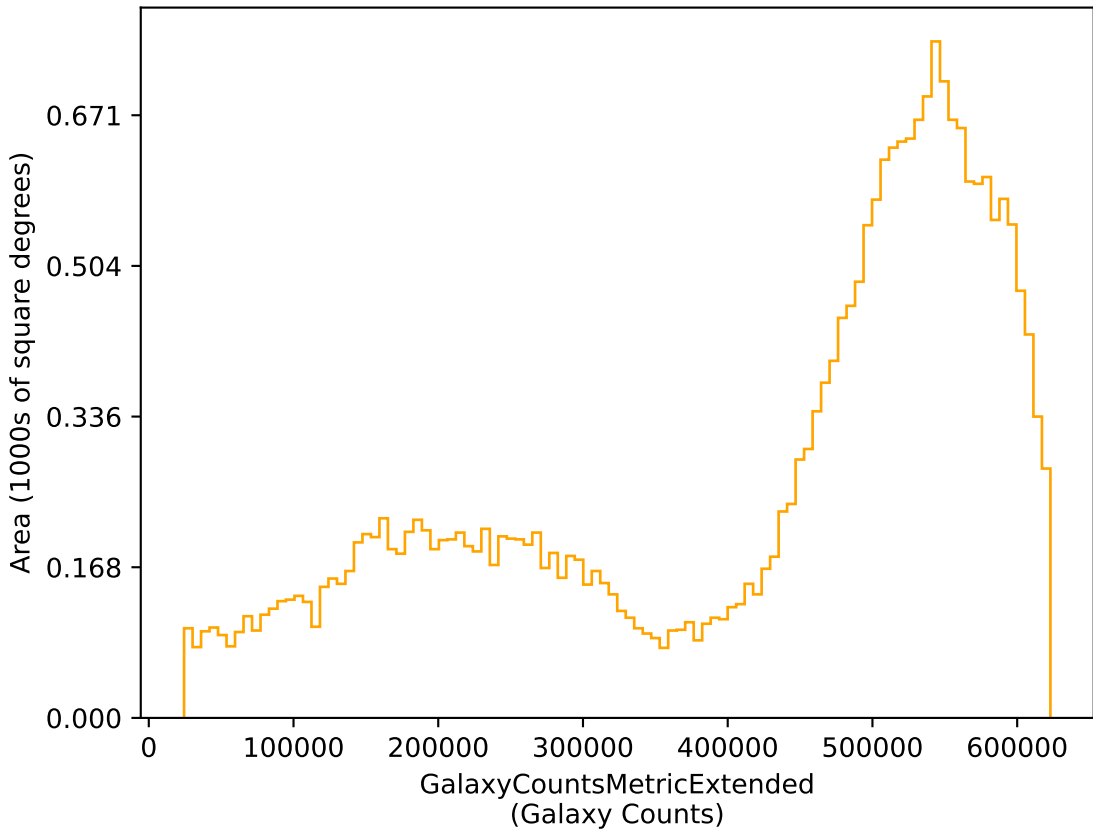
ddf_loaded_fl15_v3.4_10yrs r: GalaxyCountsMetricExtended
