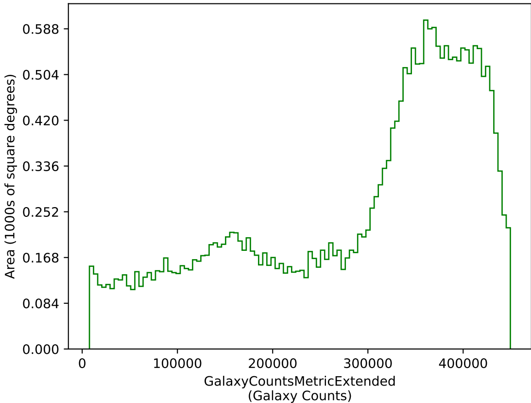
ddf_loaded_fl15_v3.4_10yrs g: GalaxyCountsMetricExtended
