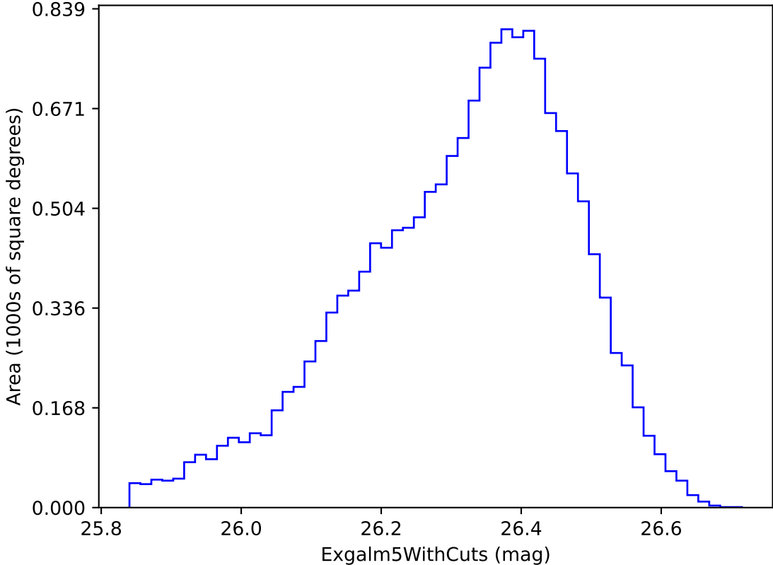
ddf_loaded_fl15_v3.4_10yrs i band non-DD year 9: ExgalM5WithCuts
