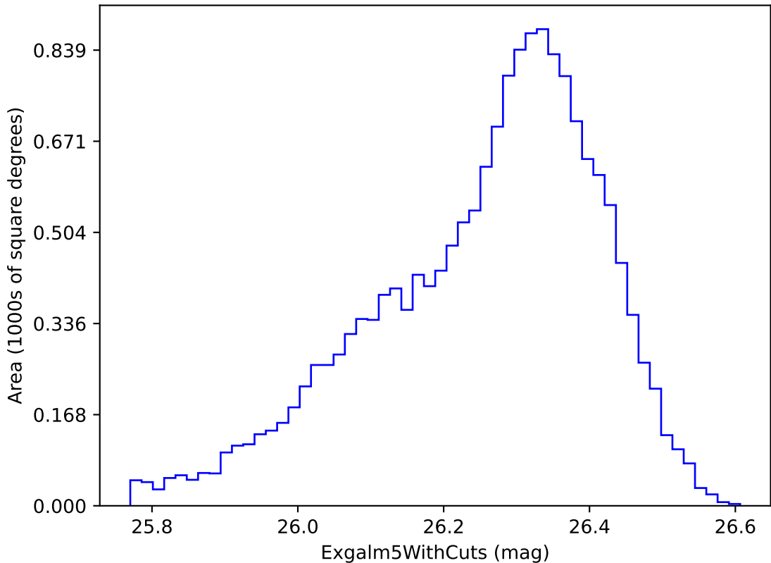
ddf_loaded_fl15_v3.4_10yrs i band non-DD year 8: ExgalM5WithCuts
