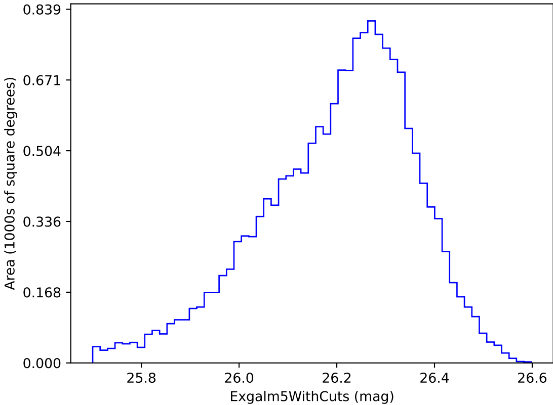
ddf_loaded_fl15_v3.4_10yrs i band non-DD year 7: ExgalM5WithCuts
