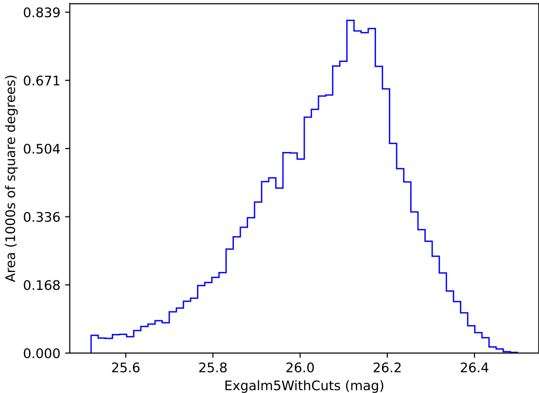
ddf_loaded_fl15_v3.4_10yrs i band non-DD year 5: ExgalM5WithCuts
