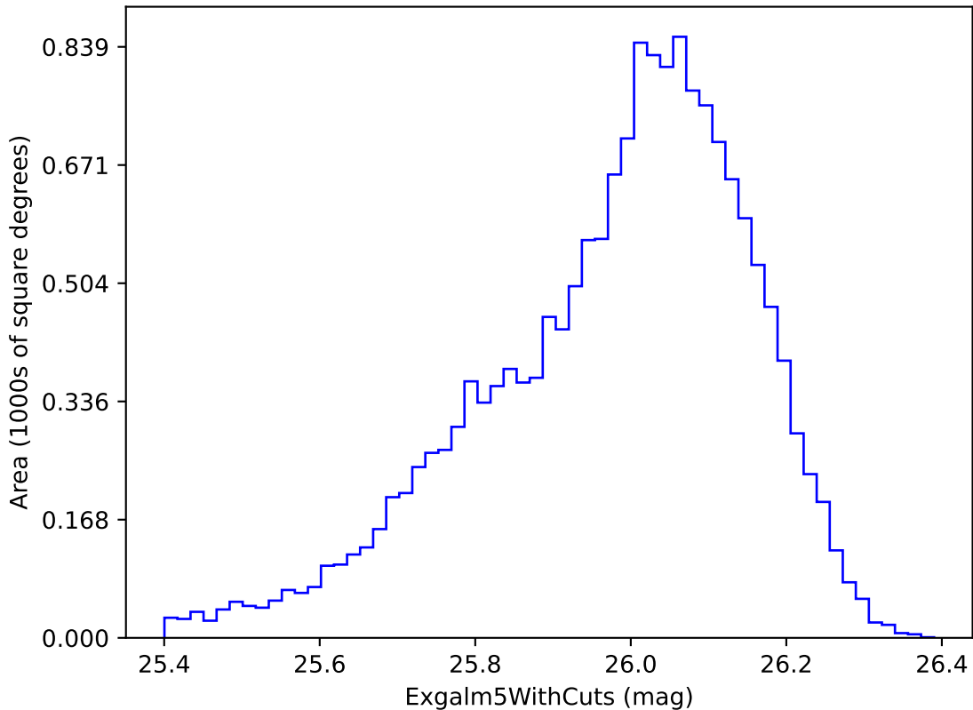
ddf_loaded_fl15_v3.4_10yrs i band non-DD year 4: ExgalM5WithCuts
